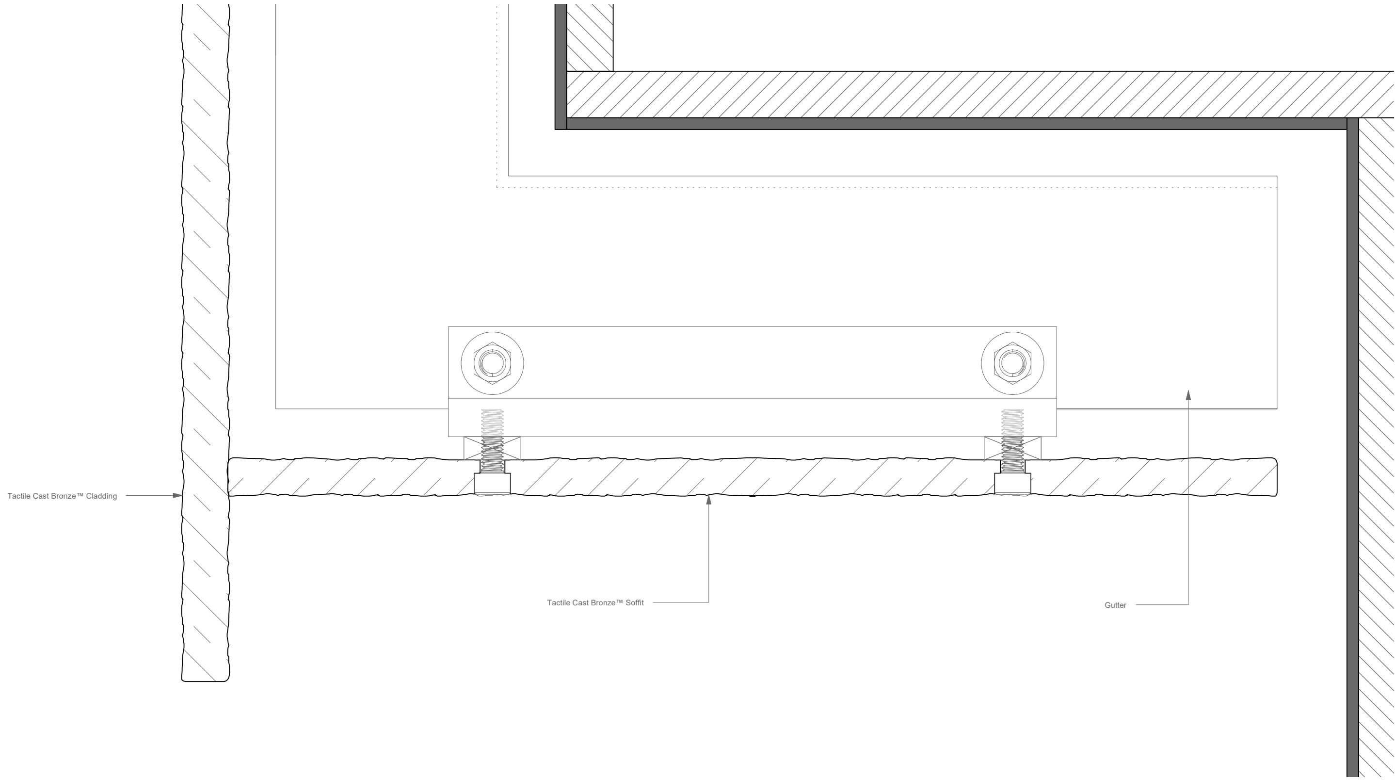
1 Section Detail - Soffit to Vertical Cladding - Tactile Cast Bronze™ Cladding AM-01 Scale: Full Scale
